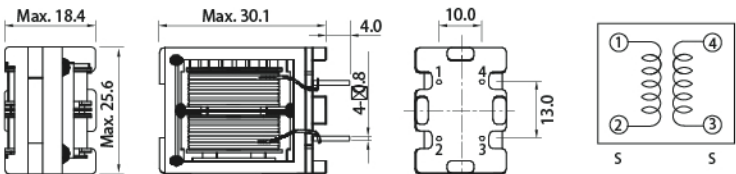
DIMENSIONS (mm)
