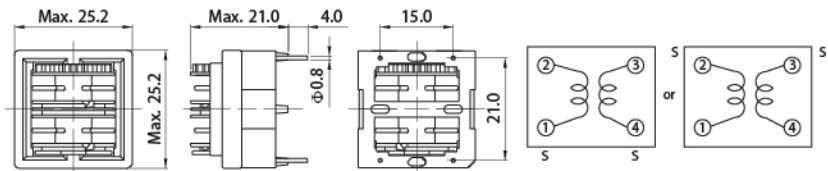
DIMENSIONS (mm)
