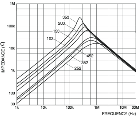
Impedance Characteristics
