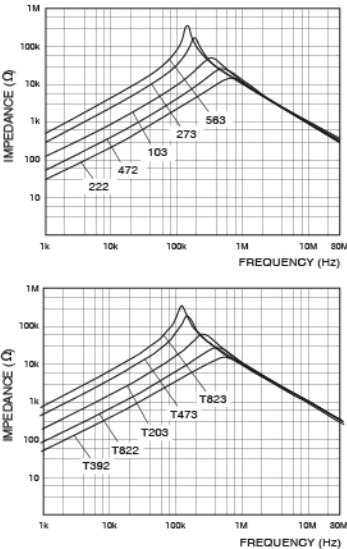
Impedance Characteristics
